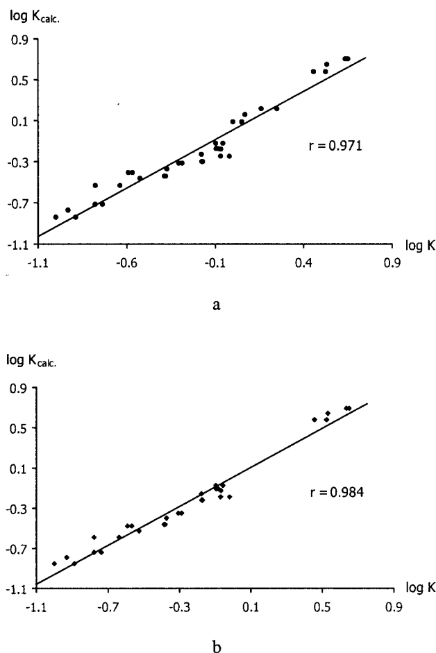
Figure 3. a: Plots of \log K_{\text{calcd.}} [calculated by applying Equation (2)] vs. \log K (experimental) for 19–23B , b: plots of \log K_{\text{calcd.}} [calculated by applying Equation (3)] vs. \log K (experimental) for 19–23B
