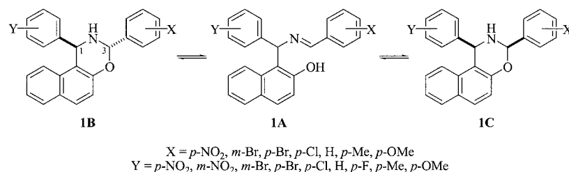
Figure 1. Ring-chain tautomeric equilibria of the 1,3-diarylnaphth[1,2- e ][1,3]oxazines
