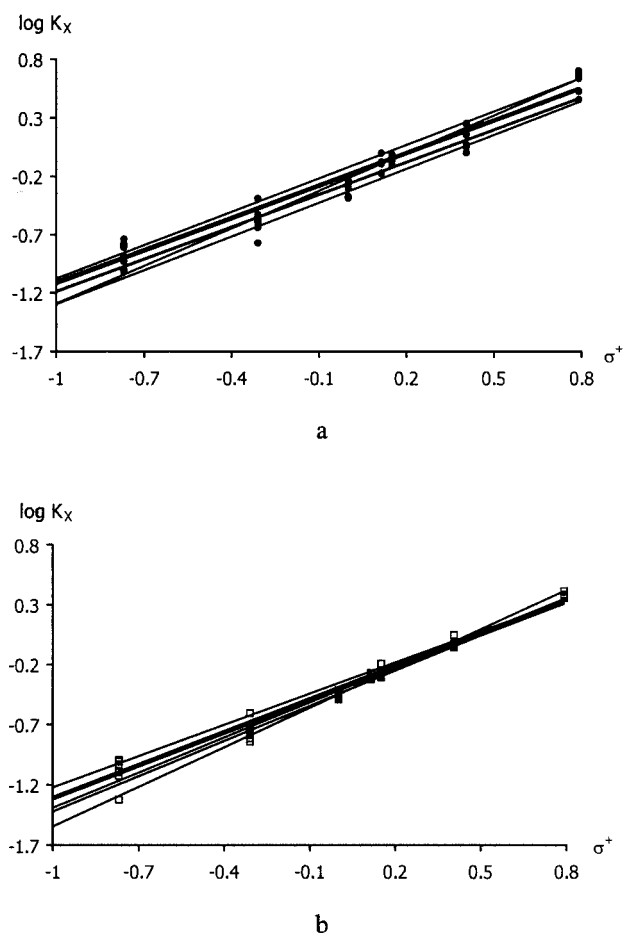
Figure 2. a: Plots of log K X for 17–23B (filled circles) vs. Hammett-Brown parameter \sigma^+ ; b: plots of log K X for 17–23C (open squares) vs. Hammett-Brown parameter \sigma^+
